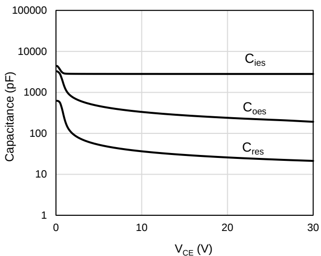
Figure 17: Capacitance Characteristics
