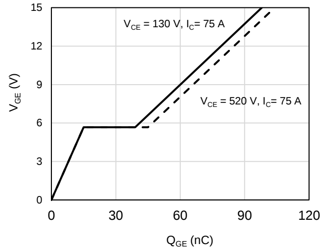
Figure 16: Gate-Charge Characteristics
